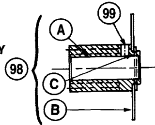
SECTION VIEW BEARING BRACKET
