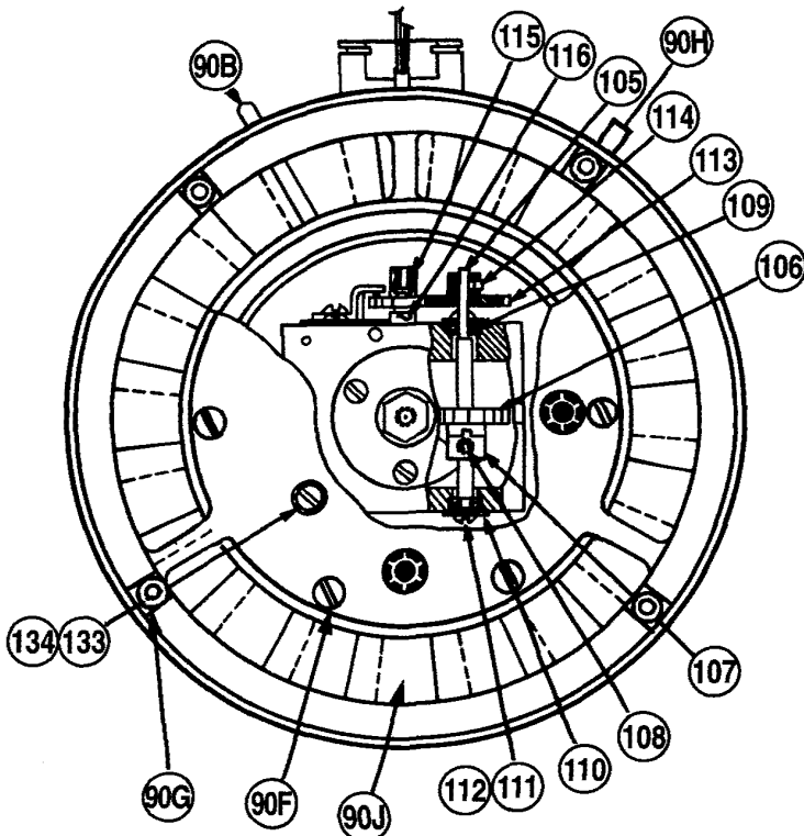
INLET VIEW
